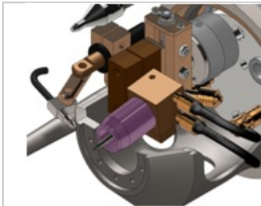
Water-cooled tilt head with adjustable wire
